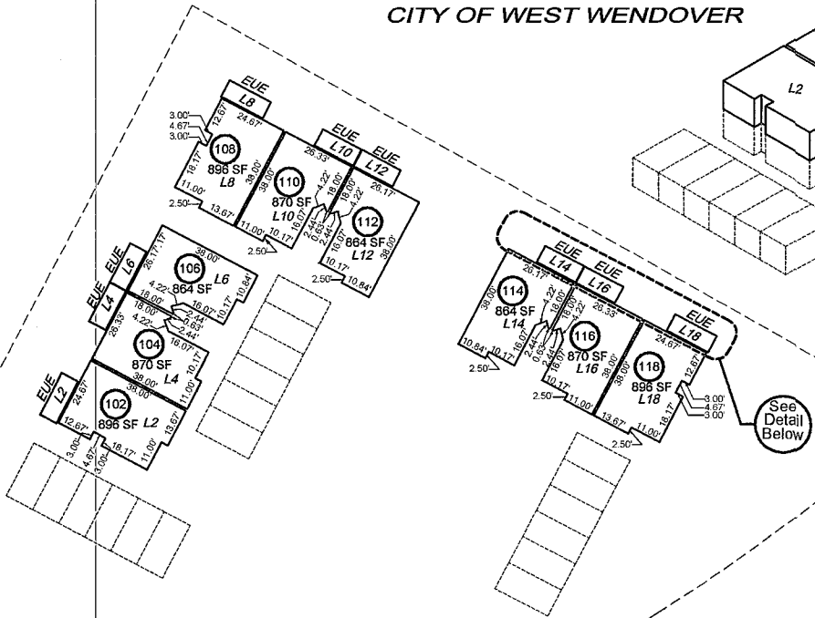
AIRSPACE ISOMETRIC
